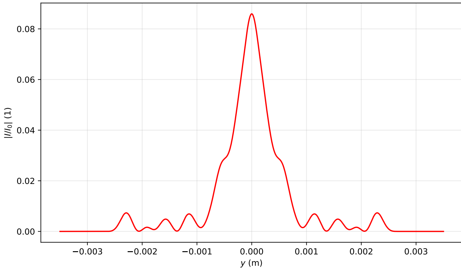
Intensity profile I(x = 0, y, z = 3.981)/I_0 , P_{in}=9.0P_{cr} , artificial time
